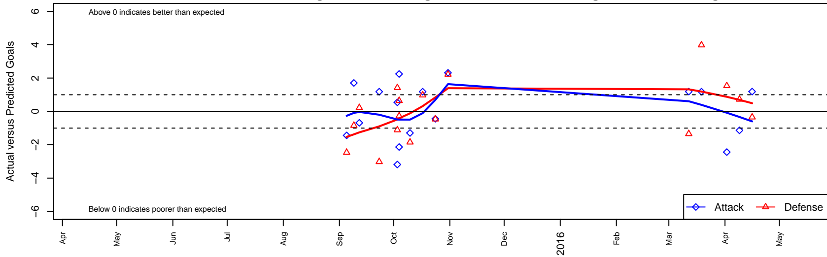
FC Nova Pink KB G04 Dots are actual minus expected GF (blue circles) and GA (red triangles). Blue line is smoothed change in attack strength. Red is smoothed change in defense strength.
